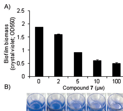
Figure 4. Dose-dependent dispersal of P. aeruginosa biofilms by 7 . A) P. aeruginosa biofilms grown in microtiter plates with shaking at 37°C were pretreated with imipenem (0.5 \mu\text{g mL}^{-1} ) for 1 h and then exposed to various concentrations of 7 (15 min) before quantifying biofilm mass by crystal violet staining. [26] B) Stained biofilms treated with the indicated concentrations of 7 .
