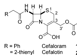
Figure 1. Chemical formulas of cephalosporin antibiotics, Cefaloram 1 and Cefalotin 2 .
