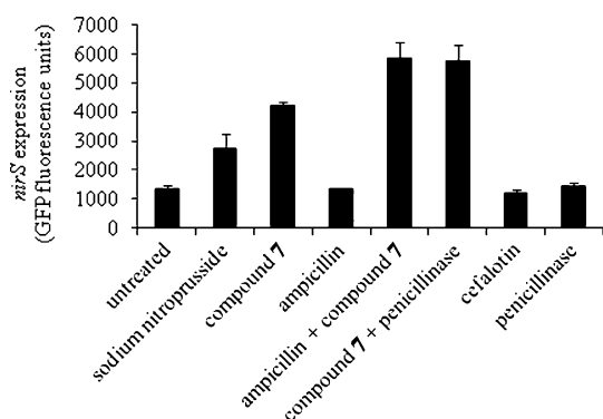
Figure 3. Compound 7 induces an NO-dependent genetic response ( nirS ) in a P. aeruginosa NSGFP reporter strain. NSGFP cells grown in the presence or absence of ampicillin (50 \mu\text{g mL}^{-1} ) were exposed to SNP (150 \mu\text{M} ), compound 7 (150 \mu\text{M} ), compound 7 (150 \mu\text{M} ) plus penicillinase (0.2 U \text{mL}^{-1} ), cefalotin 2 (150 \mu\text{M} ) or penicillinase (0.2 U \text{mL}^{-1} ), or left untreated.
