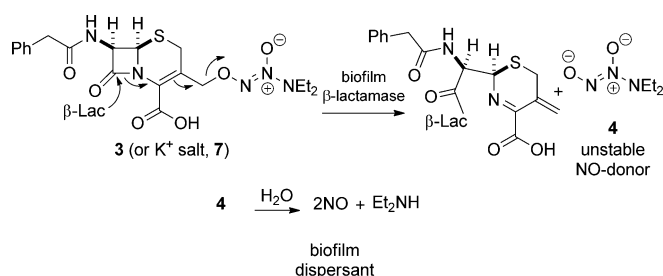
Scheme 1. Proposed mechanism of \beta -lactamase-triggered NO release and biofilm dispersion by cephalosporin-3'-diazoniumdiolate 3/7 .
