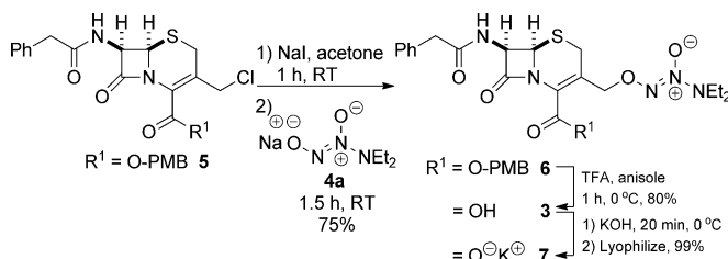
Scheme 2. Synthesis of cephalosporin-3'-diazoniumdiolate free-acid 3 and K^+ carboxylate salt 7 .
